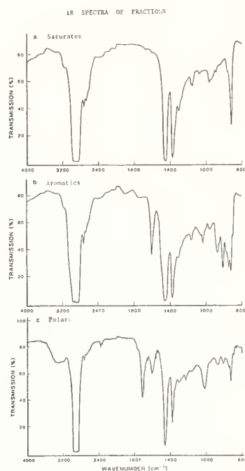
Figure 2. IR spectra of the re-refined base oil RC fractions: a) saturates b) aromatics c) polars.
